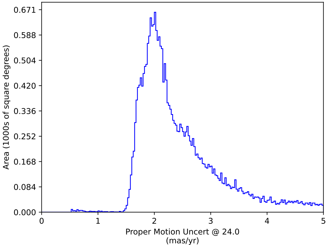
ddf_loaded_fl2_v3.4_10yrs : Proper Motion Uncert @ 24.0
