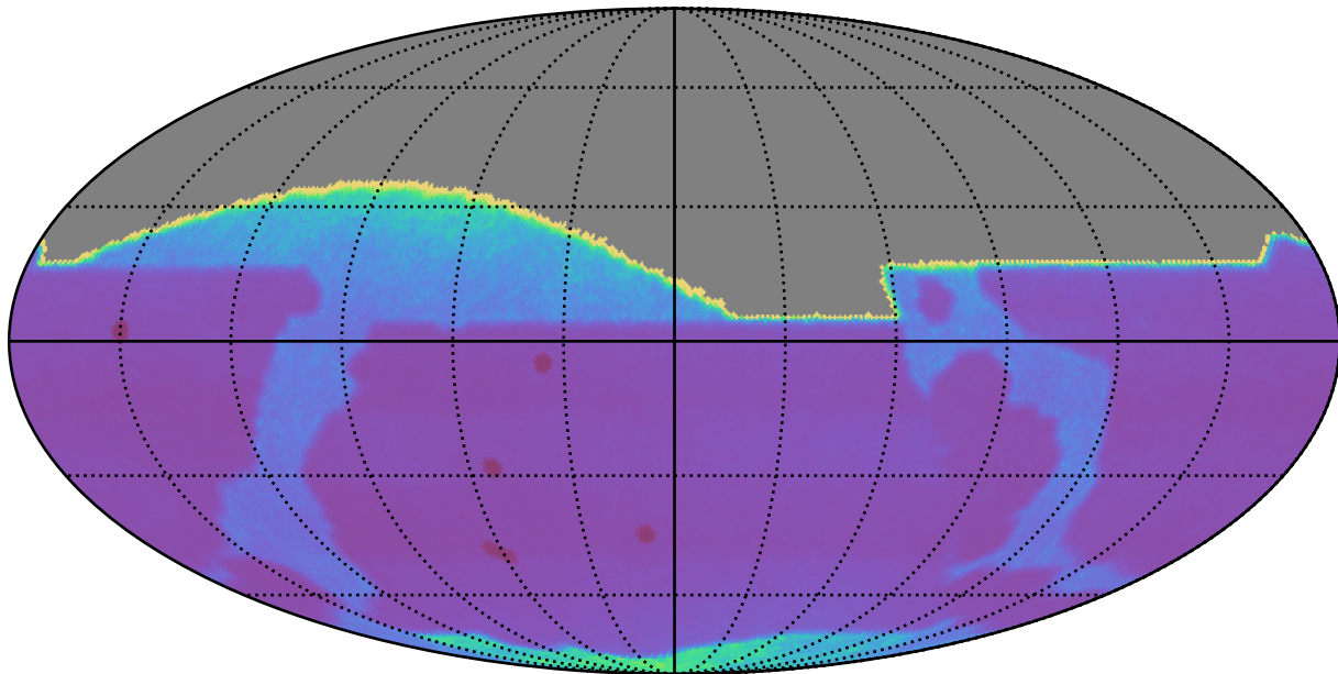
ddf_loaded_fl2_v3.4_10yrs : Proper Motion Uncert @ 20.5
