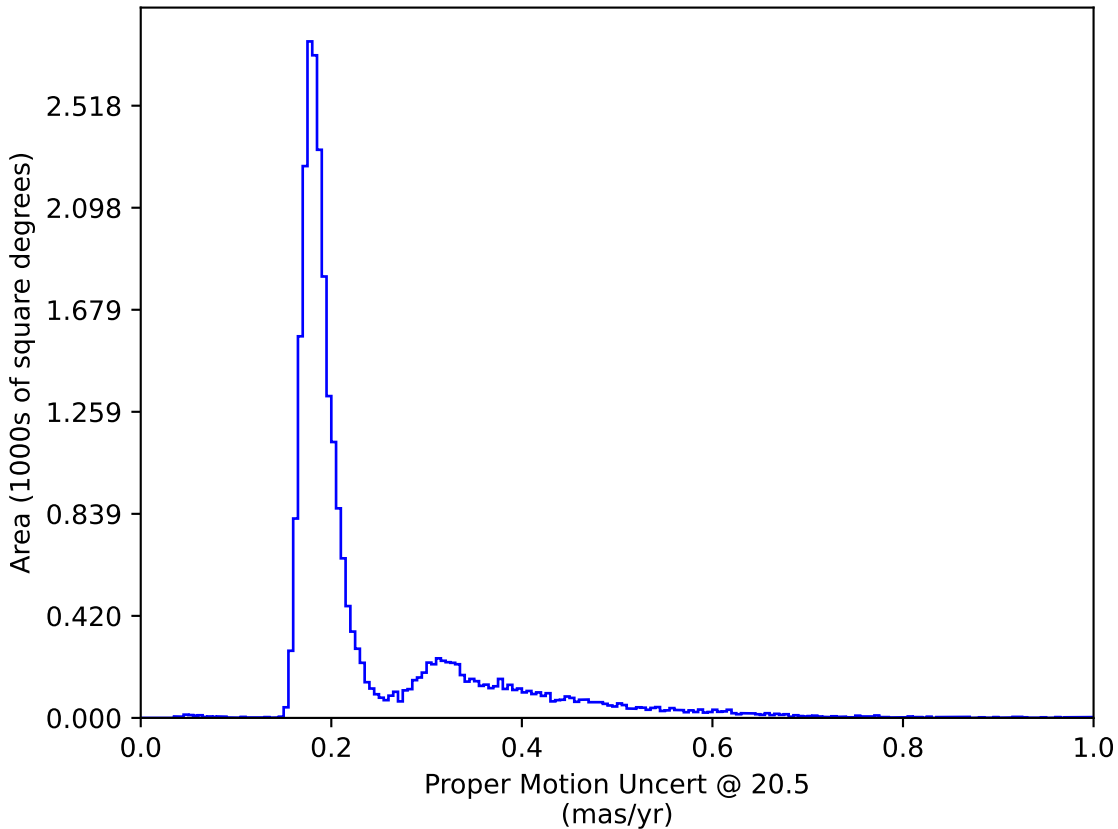
ddf_loaded_fl2_v3.4_10yrs : Proper Motion Uncert @ 20.5
