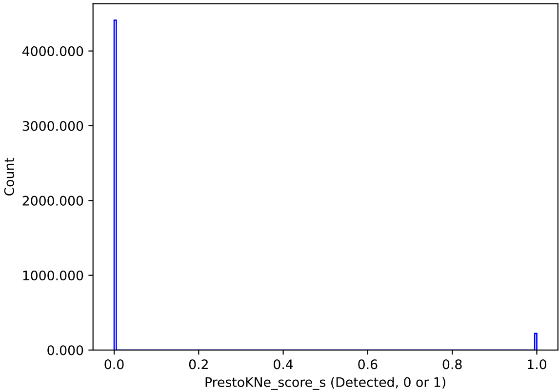
ddf_loaded_fl2_v3.4_10yrs : PrestoKNe_score_s
