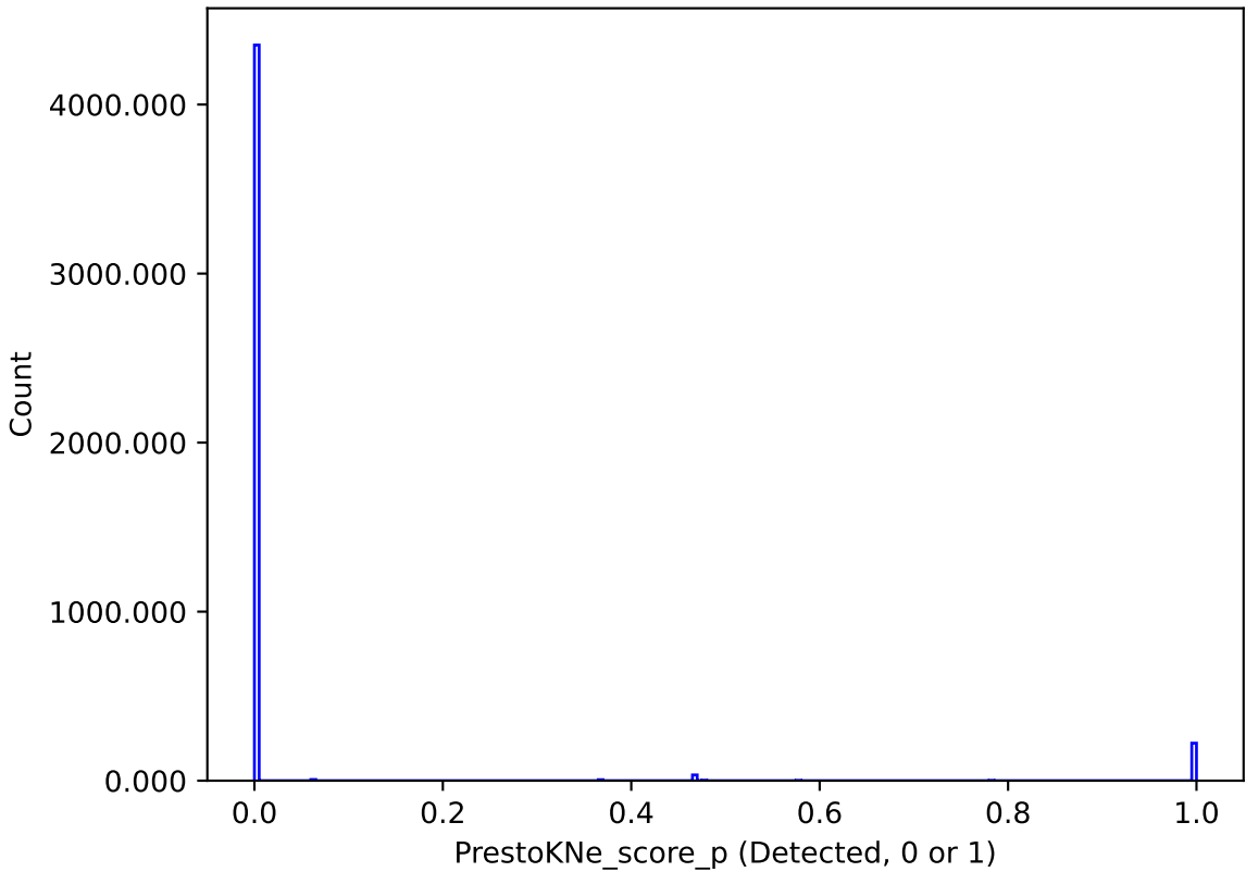
ddf_loaded_fl2_v3.4_10yrs : PrestoKNe_score_p
