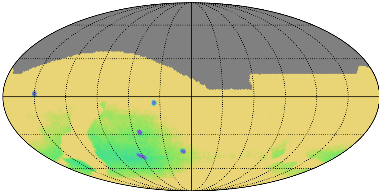
ddf_loaded_fl2_v3.4_10yrs : Parallax Uncert @ 22.4
