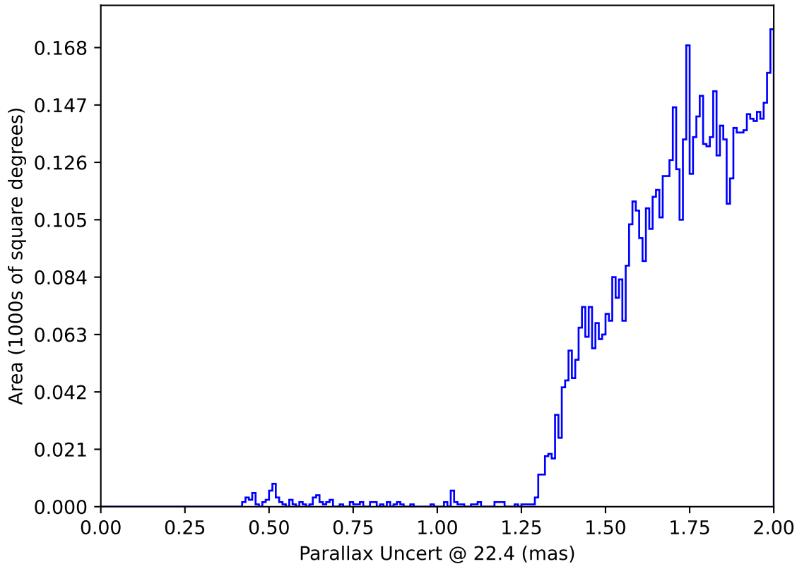
ddf_loaded_fl2_v3.4_10yrs : Parallax Uncert @ 22.4
