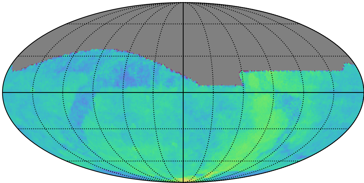
ddf_loaded_fl2_v3.4_10yrs : Parallax Coverage @ 24.0
