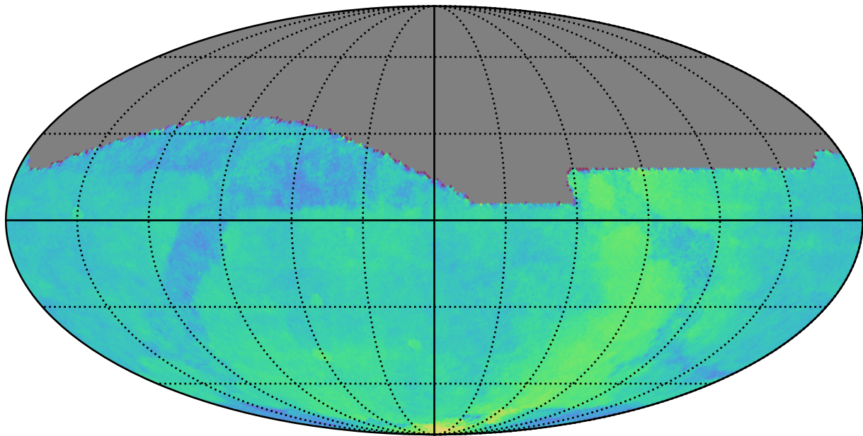
ddf_loaded_fl2_v3.4_10yrs : Parallax Coverage @ 22.4
