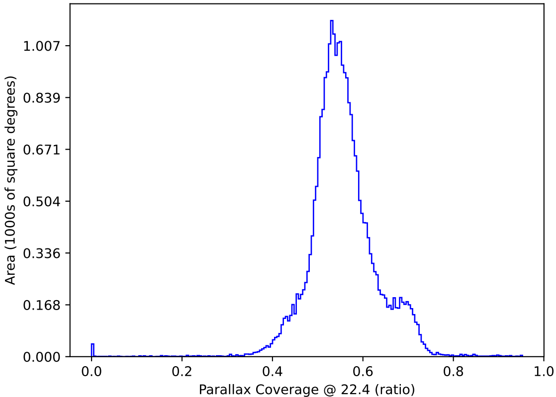
ddf_loaded_fl2_v3.4_10yrs : Parallax Coverage @ 22.4
