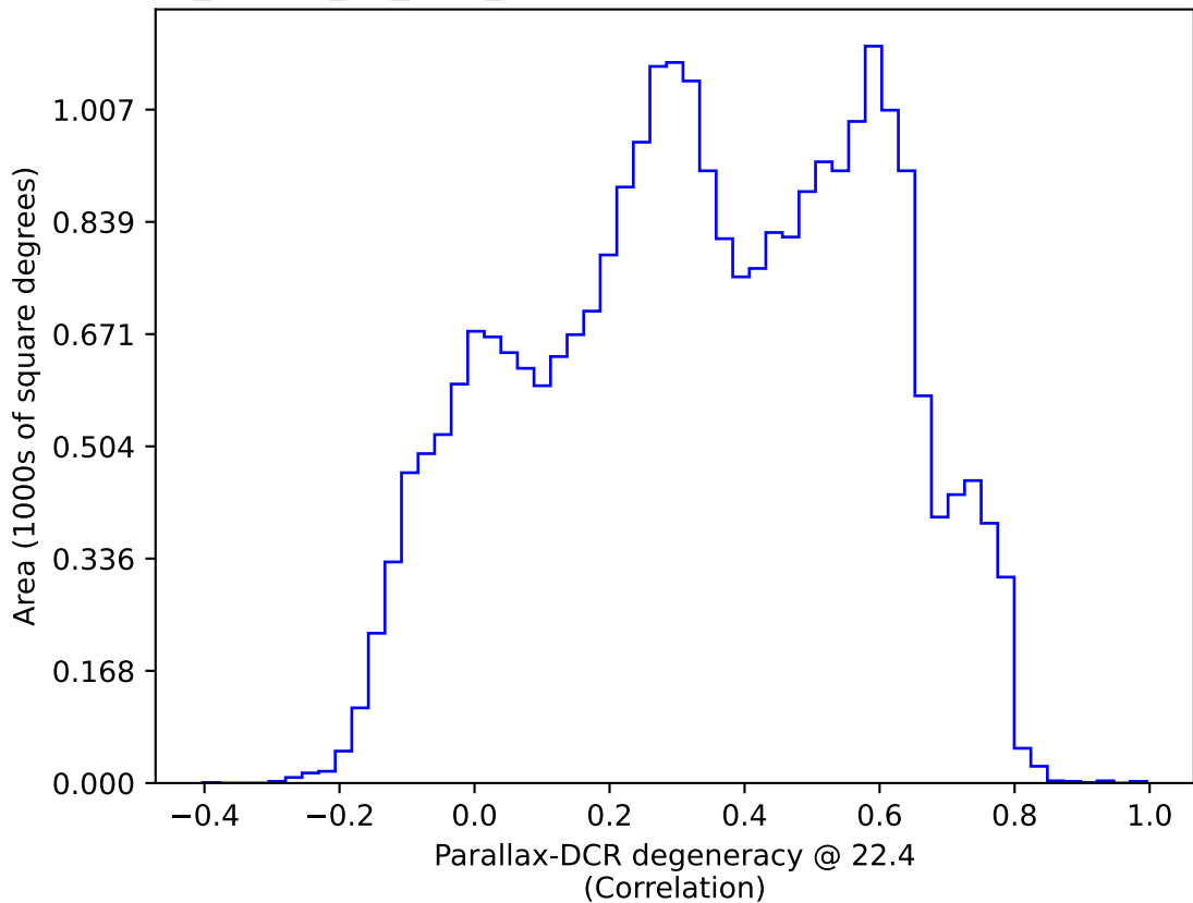
ddf_loaded_fl2_v3.4_10yrs : Parallax-DCR degeneracy @ 22.4
