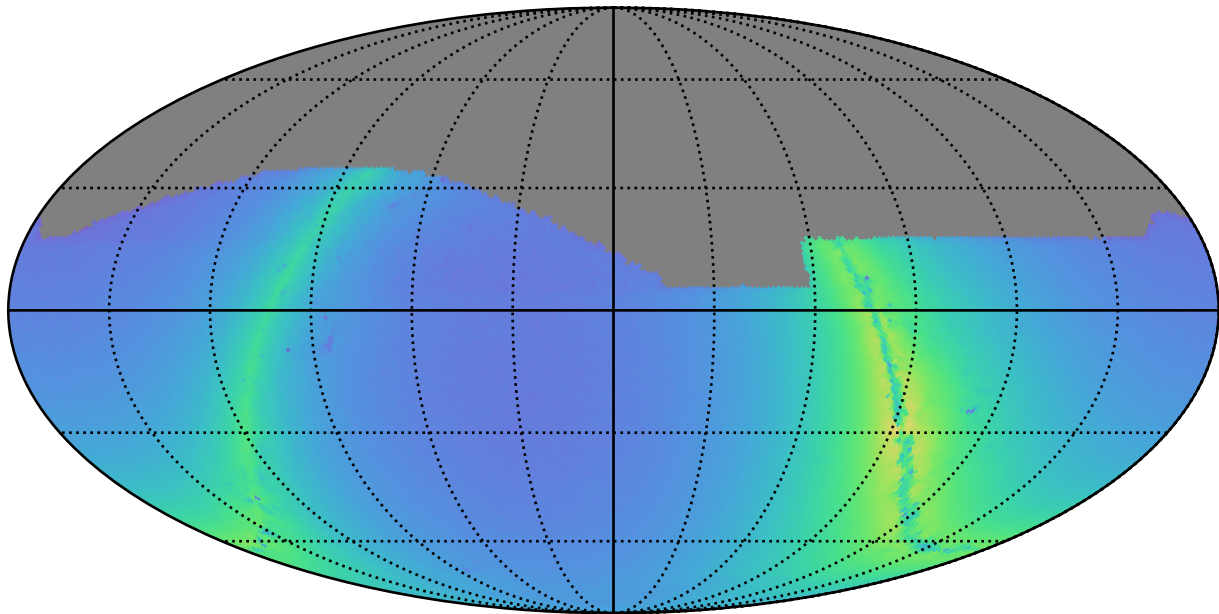
ddf_loaded_fl2_v3.4_10yrs z: Nstars_no_crowding
