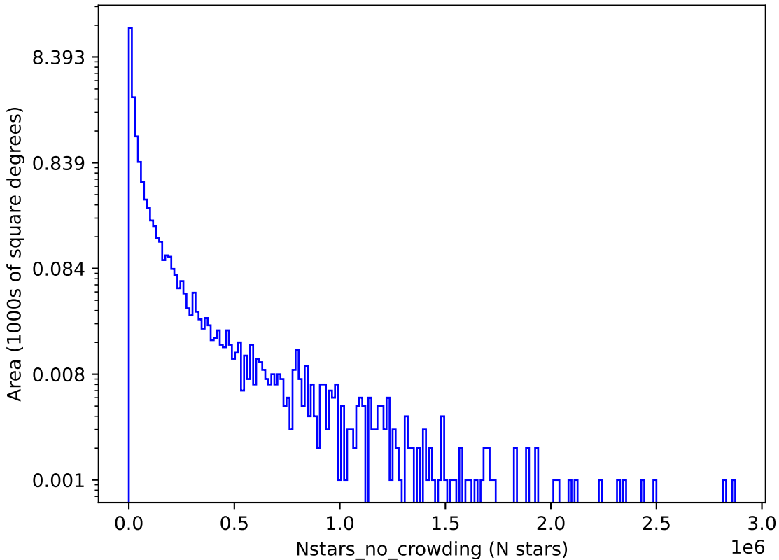
ddf_loaded_fl2_v3.4_10yrs u: Nstars_no_crowding
