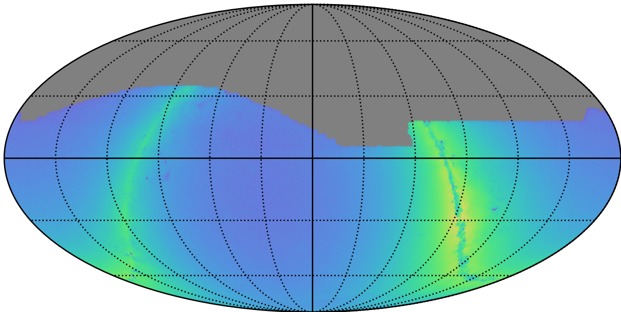
ddf_loaded_fl2_v3.4_10yrs r: Nstars_no_crowding
