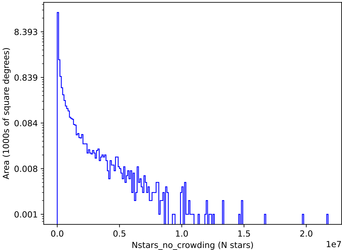
ddf_loaded_fl2_v3.4_10yrs r: Nstars_no_crowding
