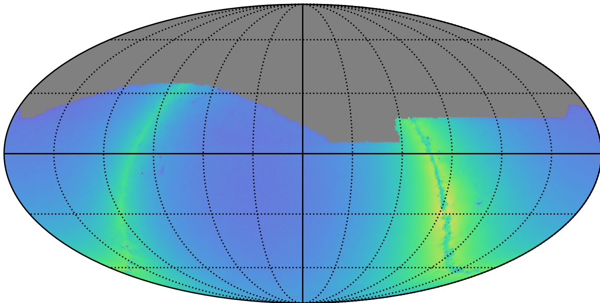
ddf_loaded_fl2_v3.4_10yrs i: Nstars_no_crowding
