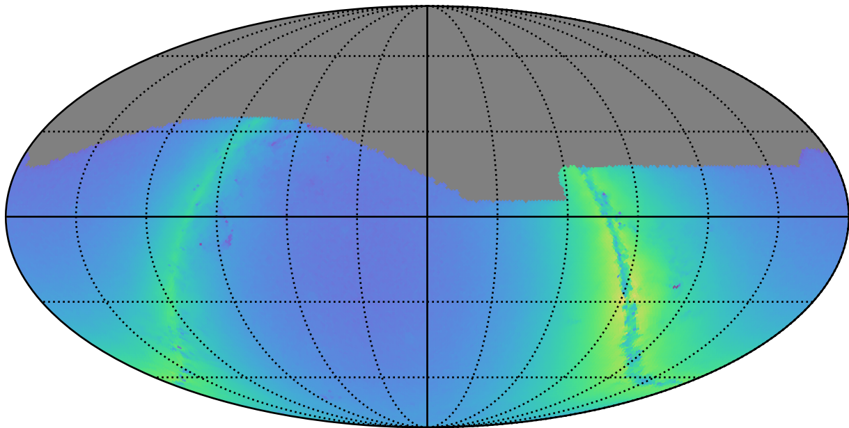
ddf_loaded_fl2_v3.4_10yrs g: Nstars_no_crowding
