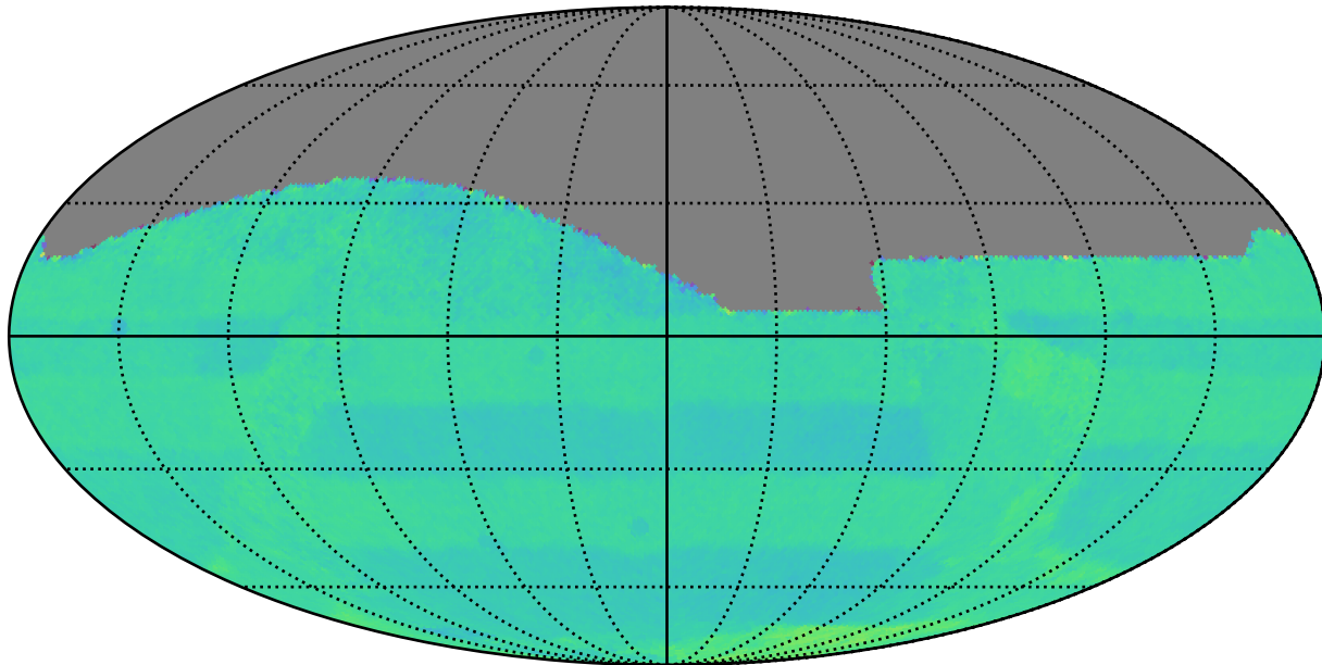
ddf_loaded_fl2_v3.4_10yrs : Normalized Proper Motion Uncert @ 20.5
