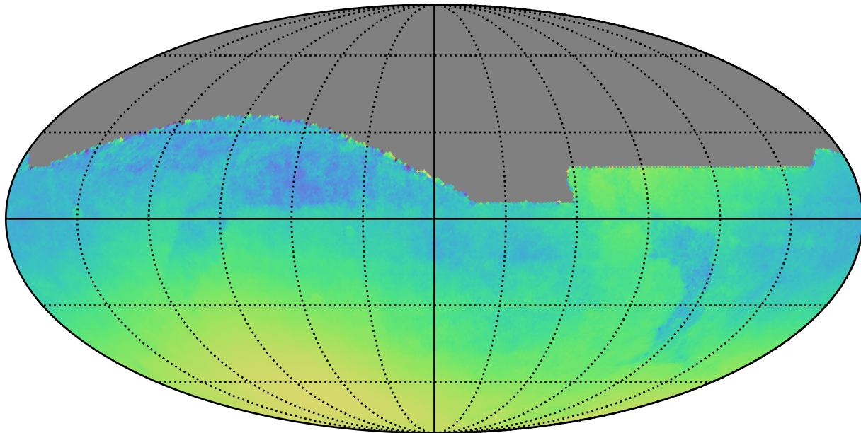
ddf_loaded_fl2_v3.4_10yrs : Normalized Parallax Uncert @ 24.0
