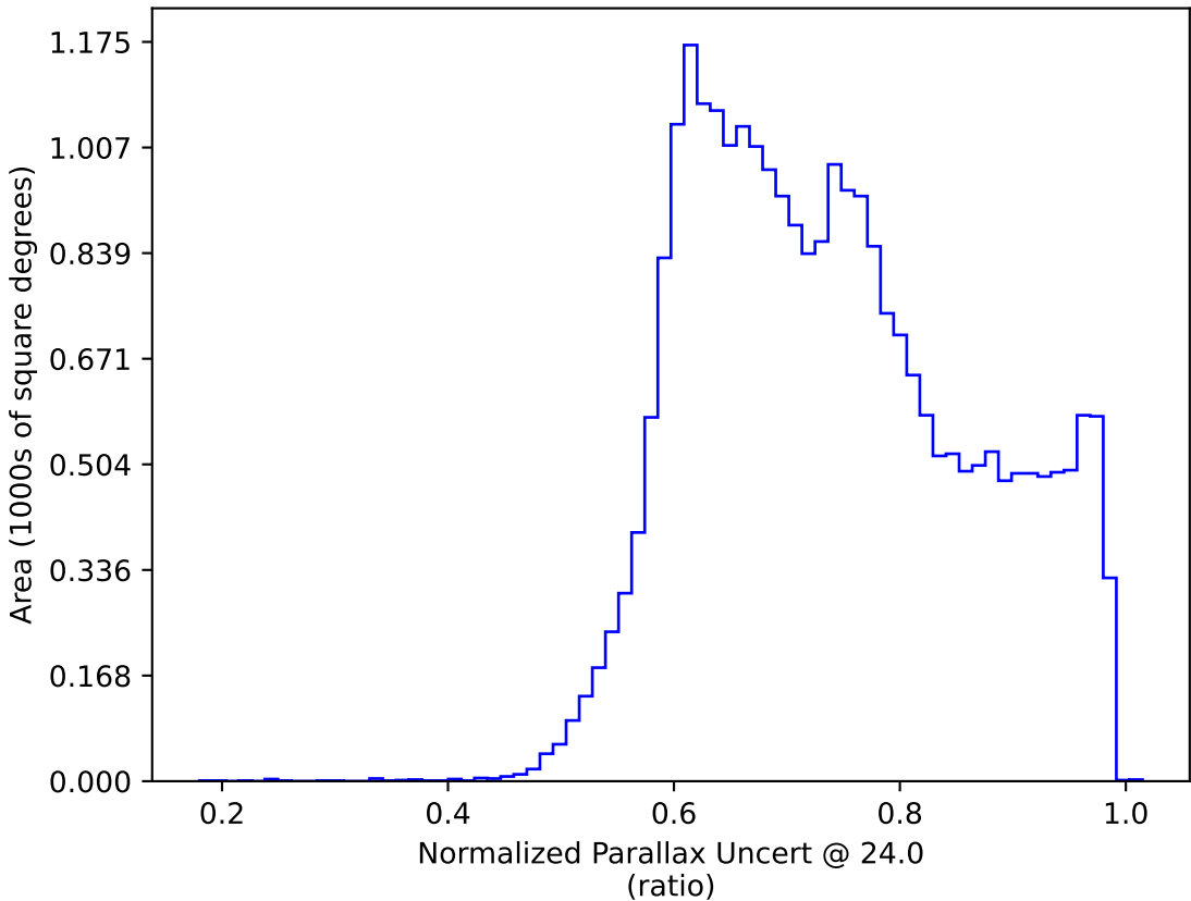
ddf_loaded_fl2_v3.4_10yrs : Normalized Parallax Uncert @ 24.0
