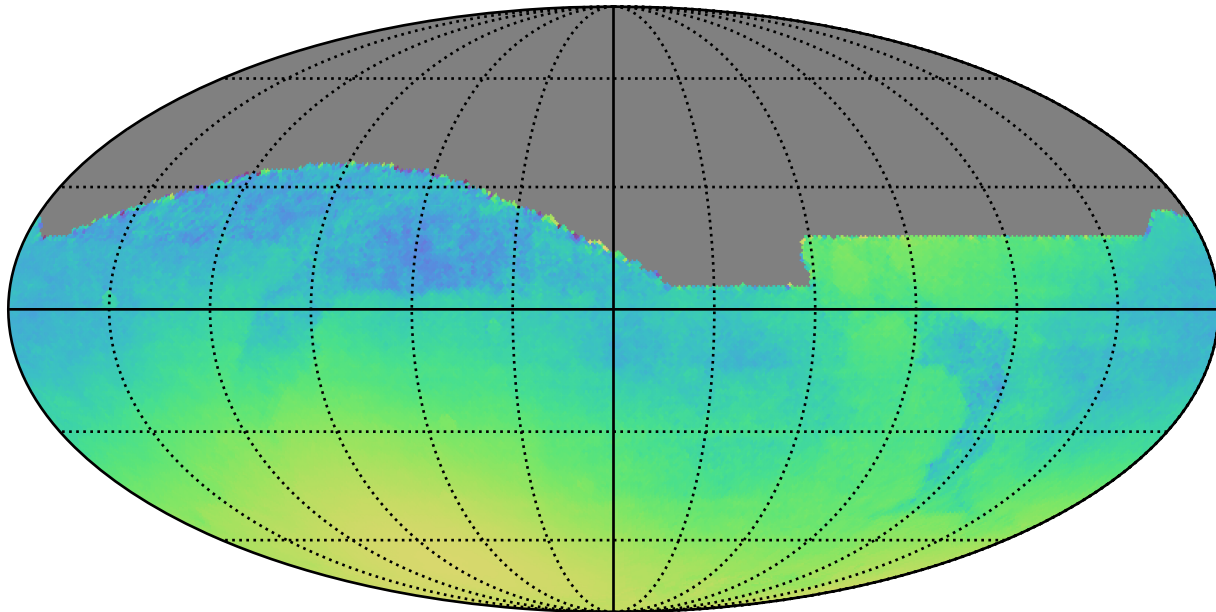
ddf_loaded_fl2_v3.4_10yrs : Normalized Parallax Uncert @ 22.4
