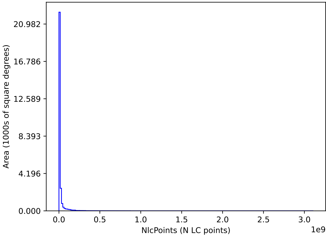
ddf_loaded_fl2_v3.4_10yrs : NlcPoints
