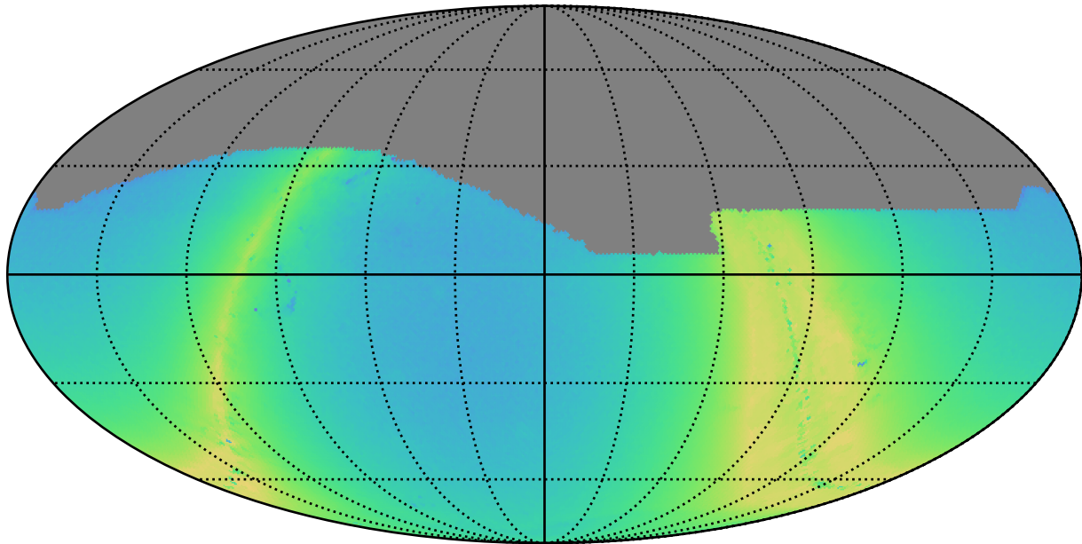
ddf_loaded_fl2_v3.4_10yrs r: N stars to Precision 0.20
