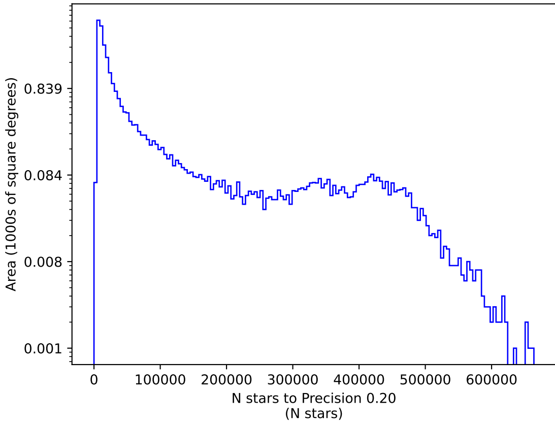
ddf_loaded_fl2_v3.4_10yrs r: N stars to Precision 0.20
