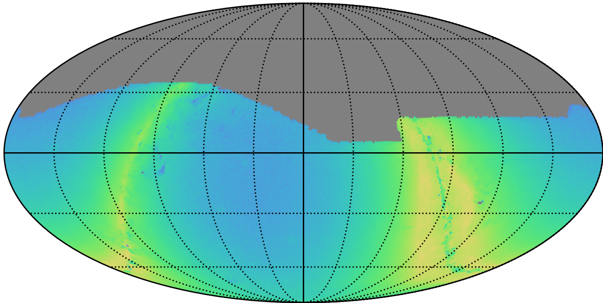
ddf_loaded_fl2_v3.4_10yrs g: N stars to Precision 0.20
