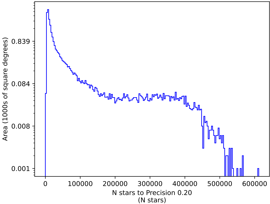
ddf_loaded_fl2_v3.4_10yrs g: N stars to Precision 0.20
