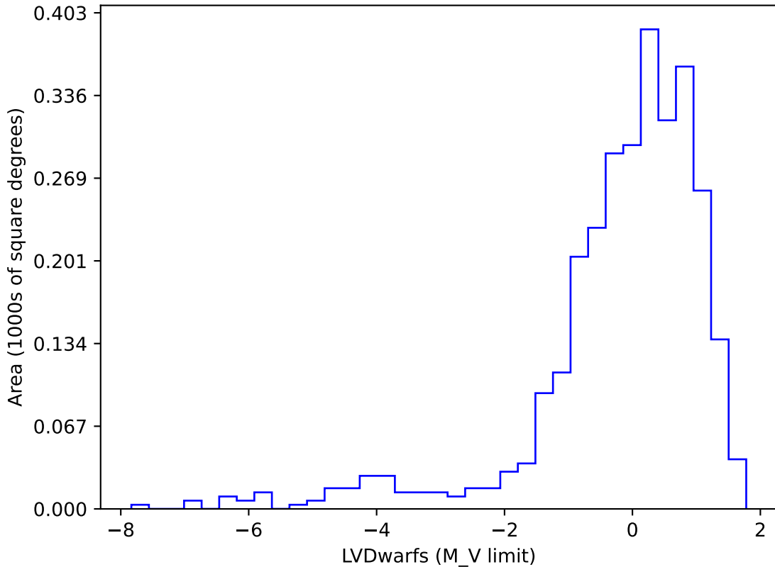
ddf_loaded_fl2_v3.4_10yrs gi SCP: LVDwarfs
