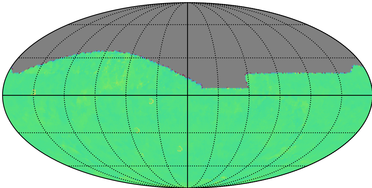
ddf_loaded_fl2_v3.4_10yrs z: Kuiper rotTelPos
