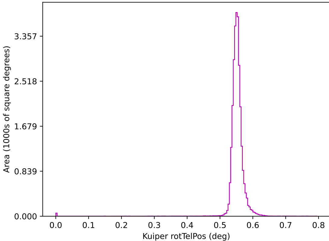
ddf_loaded_fl2_v3.4_10yrs z: Kuiper rotTelPos
