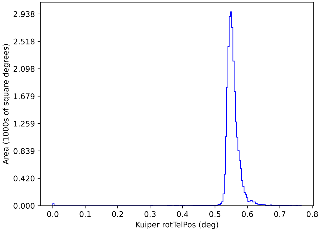
ddf_loaded_fl2_v3.4_10yrs y: Kuiper rotTelPos
