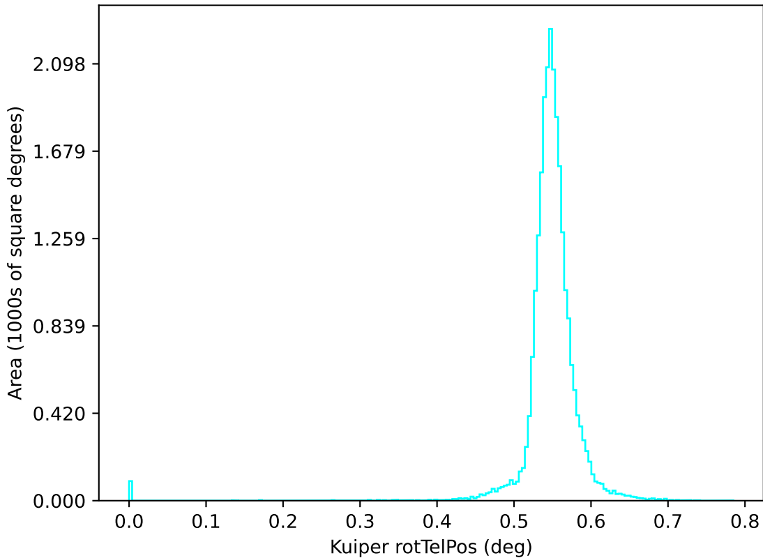
ddf_loaded_fl2_v3.4_10yrs u: Kuiper rotTelPos
