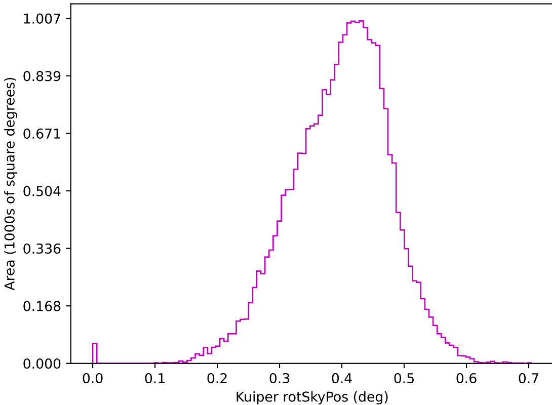
ddf_loaded_fl2_v3.4_10yrs z: Kuiper rotSkyPos
