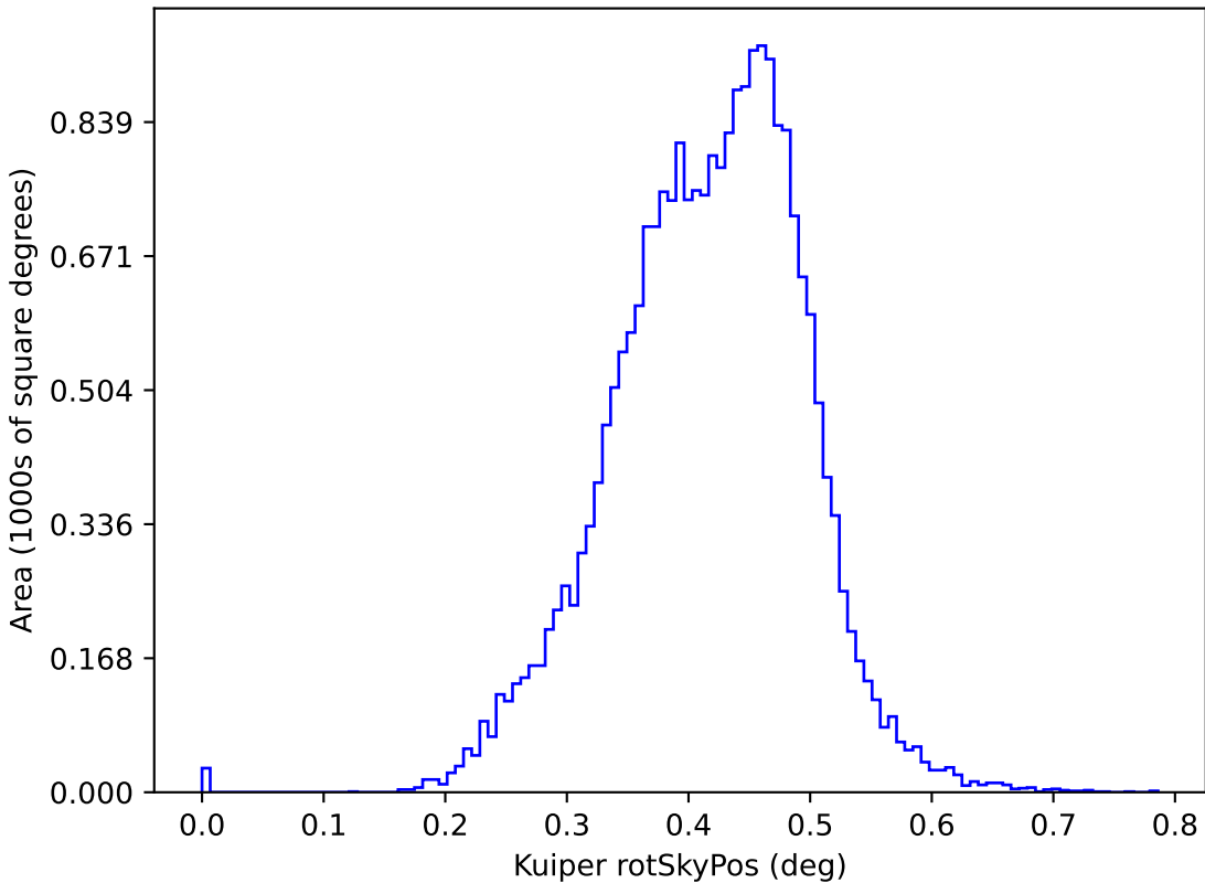
ddf_loaded_fl2_v3.4_10yrs y: Kuiper rotSkyPos
