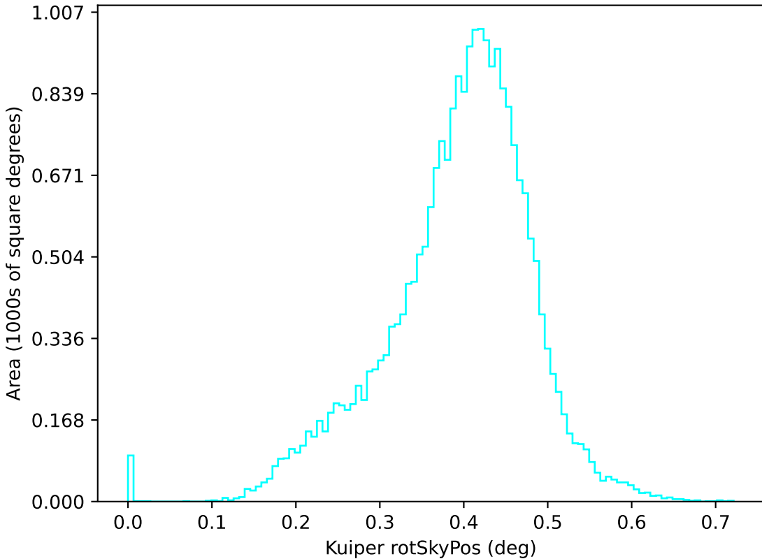
ddf_loaded_fl2_v3.4_10yrs u: Kuiper rotSkyPos
