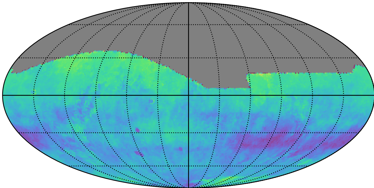
ddf_loaded_fl2_v3.4_10yrs r: Kuiper rotSkyPos
