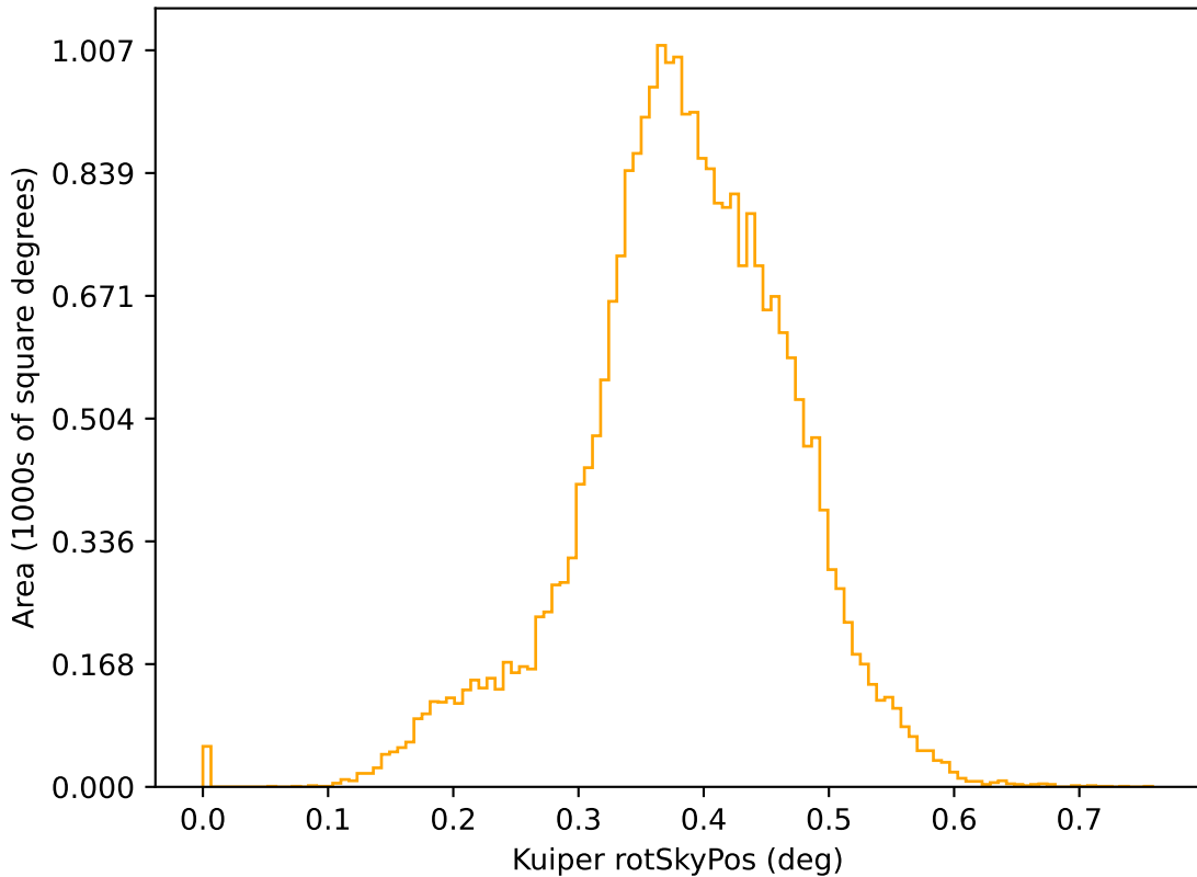
ddf_loaded_fl2_v3.4_10yrs r: Kuiper rotSkyPos
