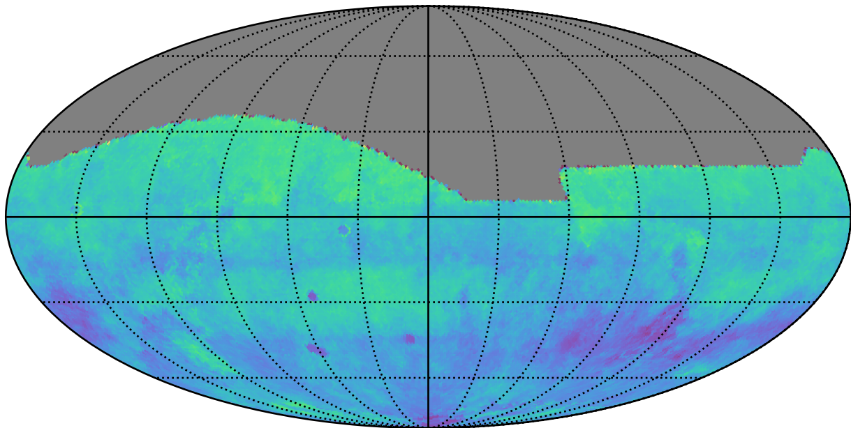
ddf_loaded_fl2_v3.4_10yrs i: Kuiper rotSkyPos
