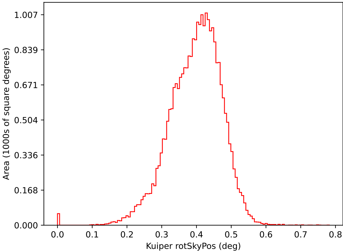
ddf_loaded_fl2_v3.4_10yrs i: Kuiper rotSkyPos
