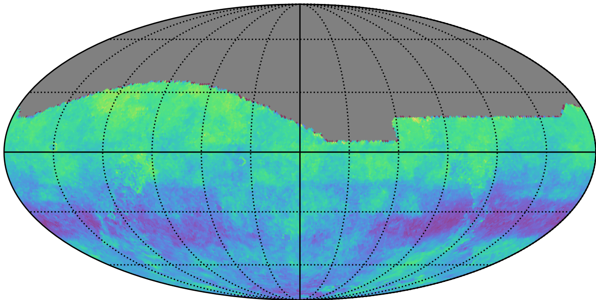
ddf_loaded_fl2_v3.4_10yrs g: Kuiper rotSkyPos
