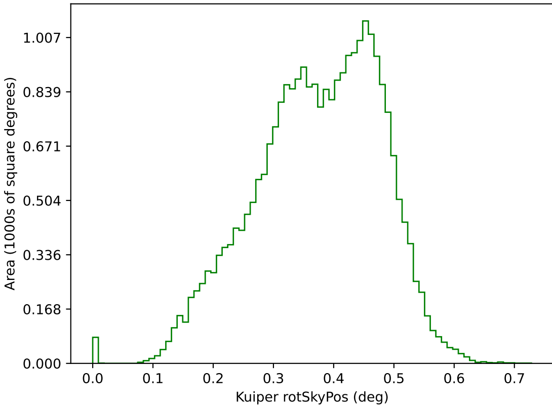
ddf_loaded_fl2_v3.4_10yrs g: Kuiper rotSkyPos
