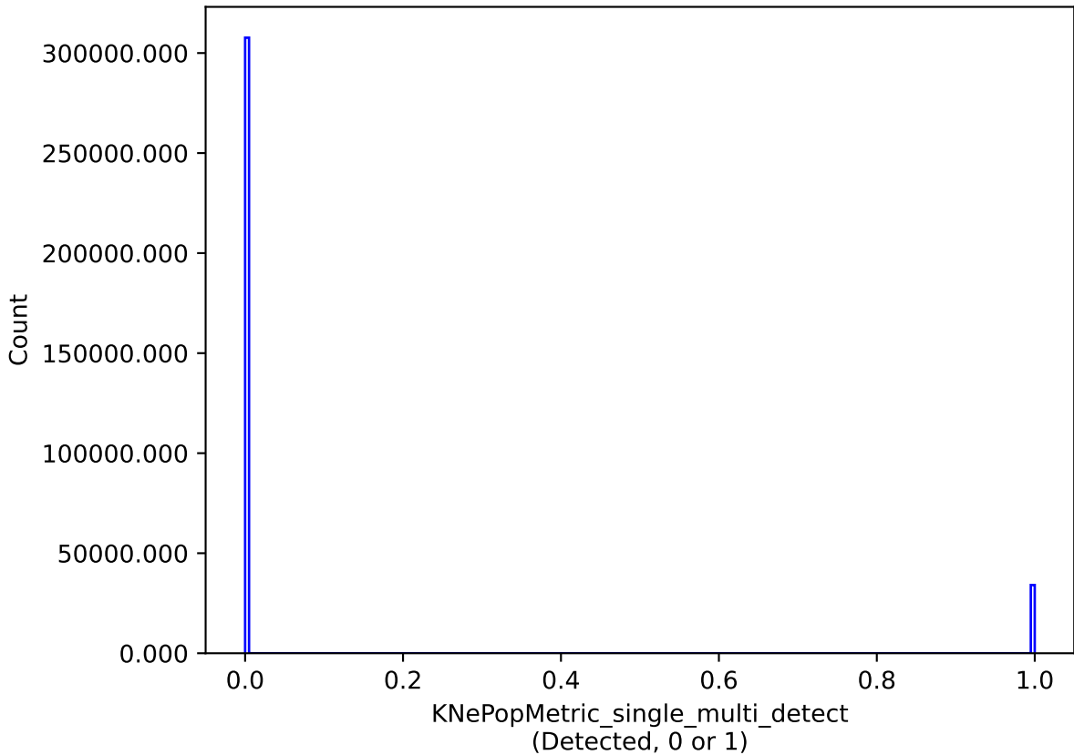
ddf_loaded_fl2_v3.4_10yrs single model: KNePopMetric_single_multi_detect
