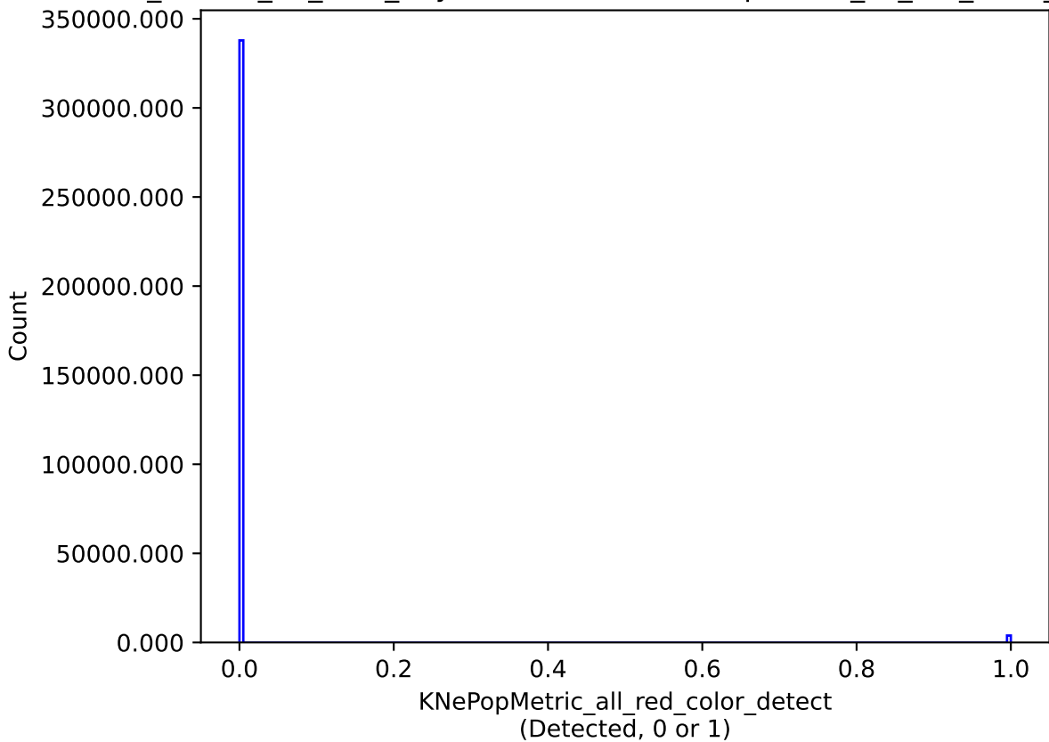
ddf_loaded_fl2_v3.4_10yrs all models: KNePopMetric_all_red_color_detect
