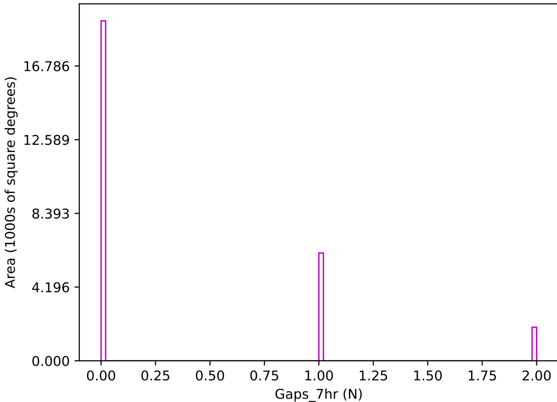
ddf_loaded_fl2_v3.4_10yrs z band: Gaps_7hr
