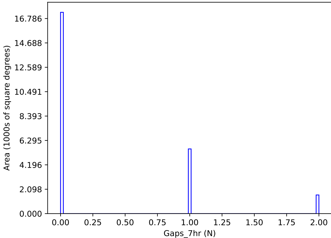
ddf_loaded_fl2_v3.4_10yrs y band: Gaps_7hr
