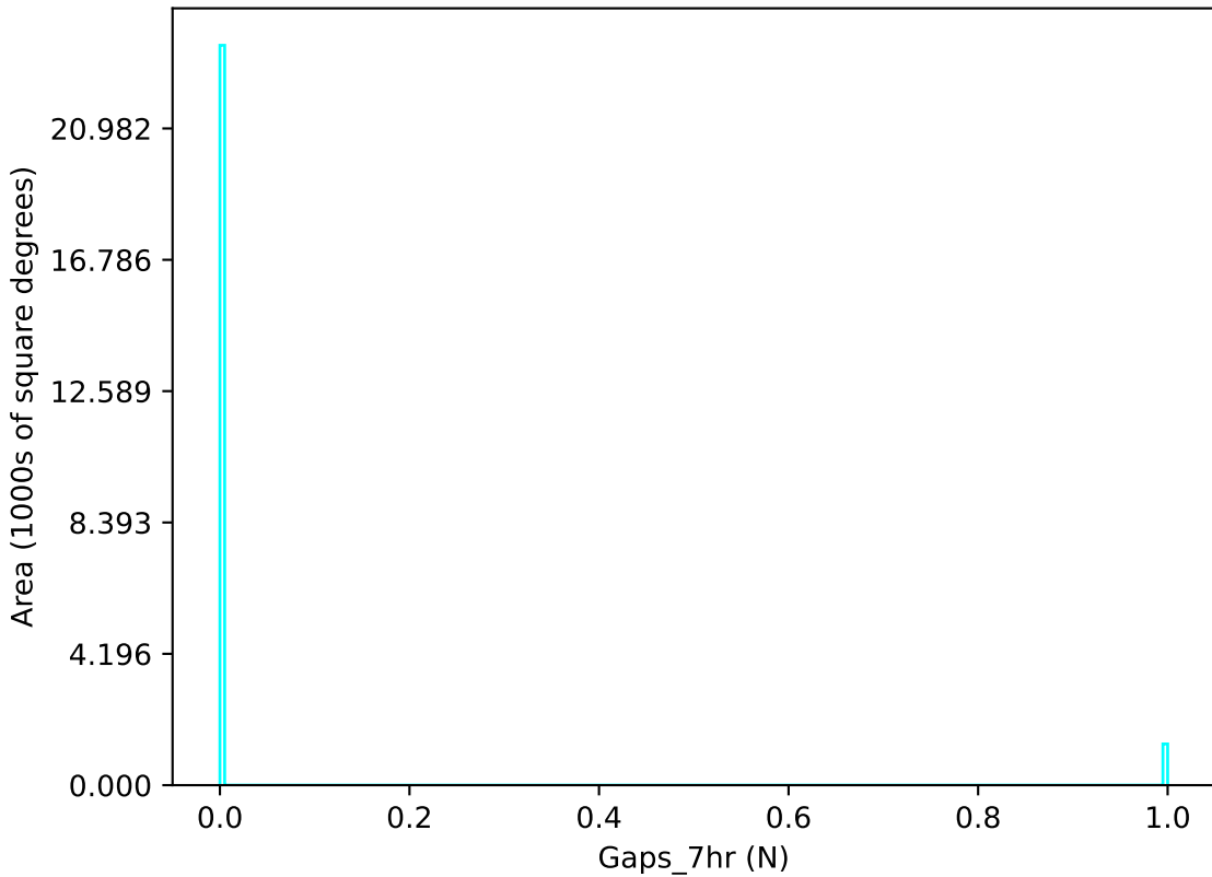
ddf_loaded_fl2_v3.4_10yrs u band: Gaps_7hr
