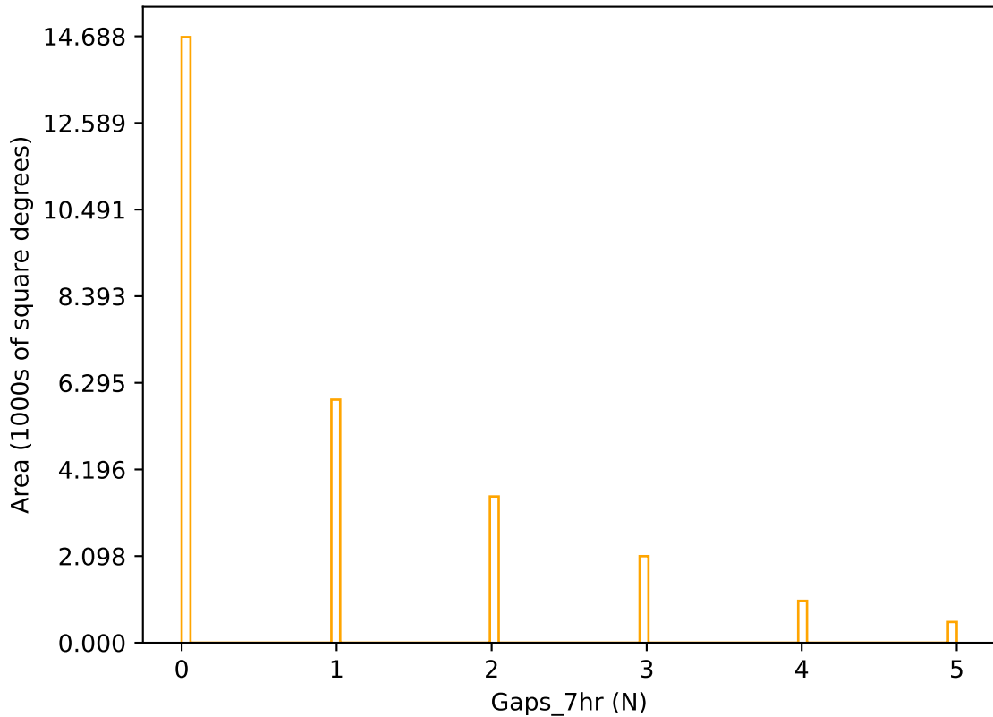
ddf_loaded_fl2_v3.4_10yrs r band: Gaps_7hr
