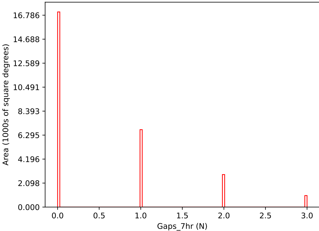
ddf_loaded_fl2_v3.4_10yrs i band: Gaps_7hr
