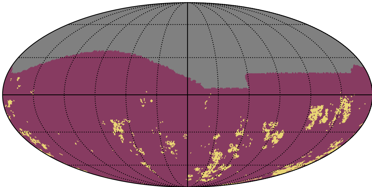
ddf_loaded_fl2_v3.4_10yrs g band: Gaps_7hr
