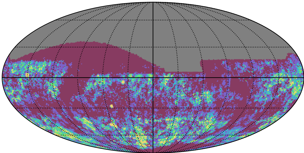
ddf_loaded_fl2_v3.4_10yrs z band: Gaps_3hr
