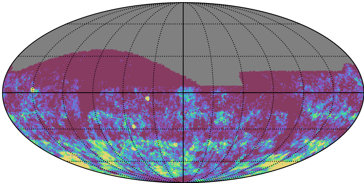
ddf_loaded_fl2_v3.4_10yrs r band: Gaps_3hr
